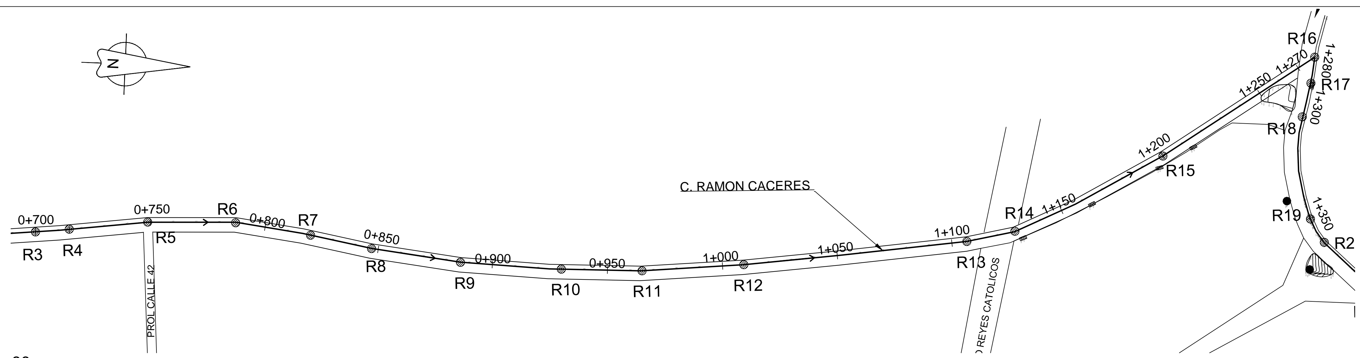
PLANTA GENERAL C/RAMON CACERES ESC.1:1000
